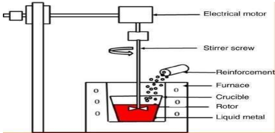
Figure2:- Stir casting
