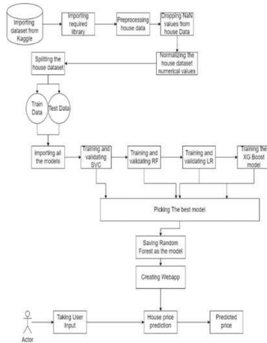
Fig 1.1 Architecture diagram
