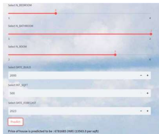
Fig.1.20 WebApp Output
