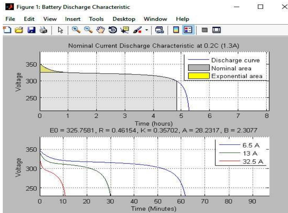
Figure 4: Battery discharge characteristic
