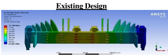
Fig.4 existing design
