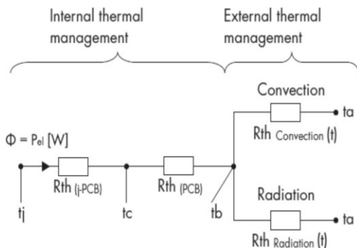
Fig.2: Internal circuite diagram of Luminaire
