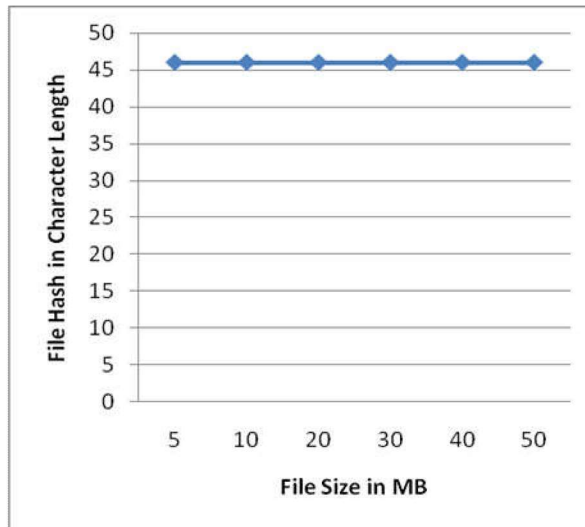
Figure 4.3. File Hash
